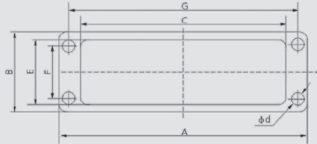
G10A, G16A, G32A开孔底座 G6B, G10B, G16B, G24B, G32B, G48B开孔底座 G10A, G16A, G32A series housings G6B, G10B, G16B, G24B, G32B, G48Bseries housings
